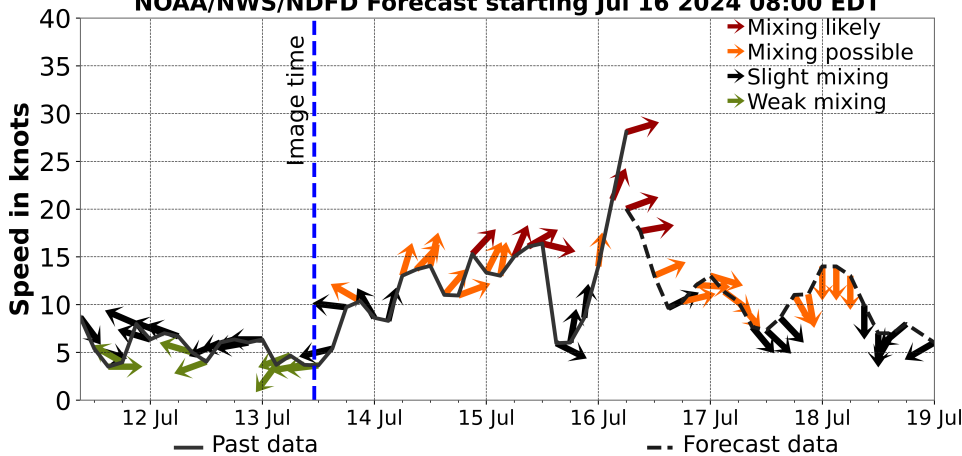
ndbc.noaa.gov Winds at South Bass Is, OH NOAA/NWS/NDFD Forecast starting Jul 16 2024 08:00 EDT
